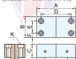
Stationary Jaw / 固定口金 (鋼製硬爪, 研磨 Hardened)
