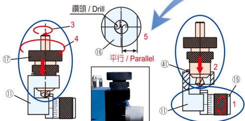
C. 如何研磨鑽頭先端角 How to grind point angle
