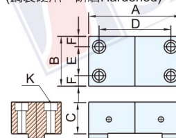
Stationary Jaw (Center-Step) 中間固定口金 (階梯) (鋼製硬爪, 研磨 Hardened)
