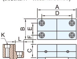
Stationary Jaw (Center) 中間固定口金 (鋼製硬爪, 研磨 Hardened)
